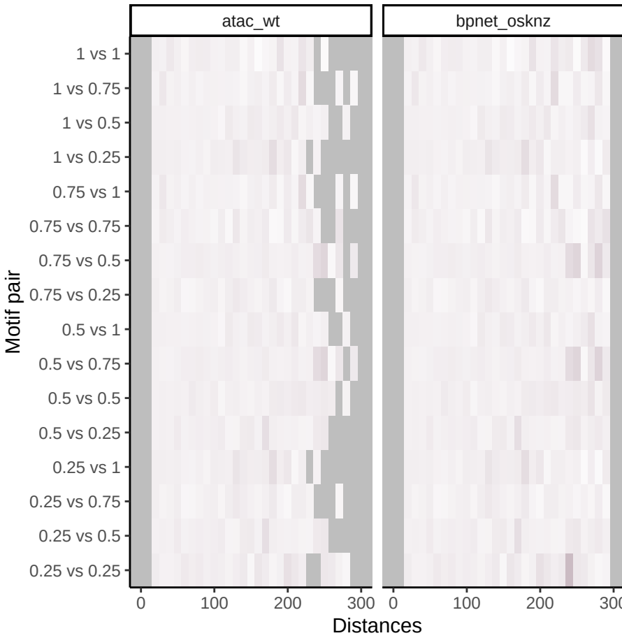
Nanog vs Oct4-Sox2
